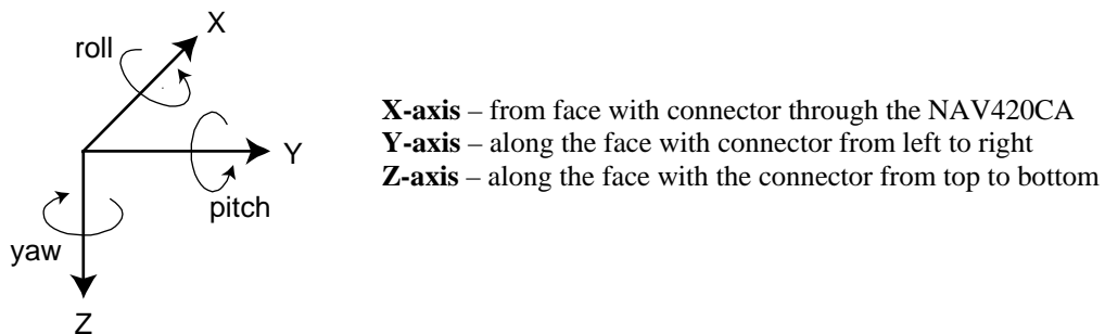
Figure 1: NAV420CA Coordinate System
